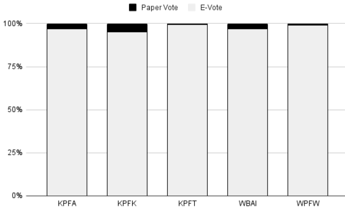
Graph 4. Percent of votes cast by paper and electronically by station
